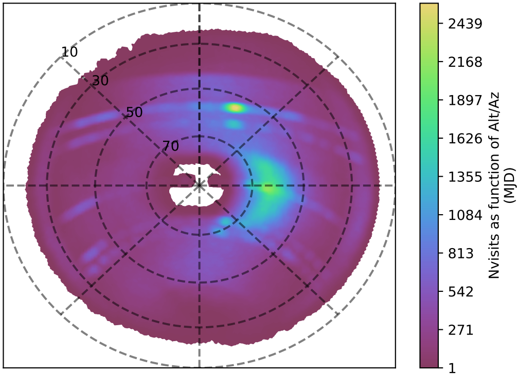
internal_u_expt60_nscale1.5v3.4_10yrs z band: Nvisits as function of Alt/Az
