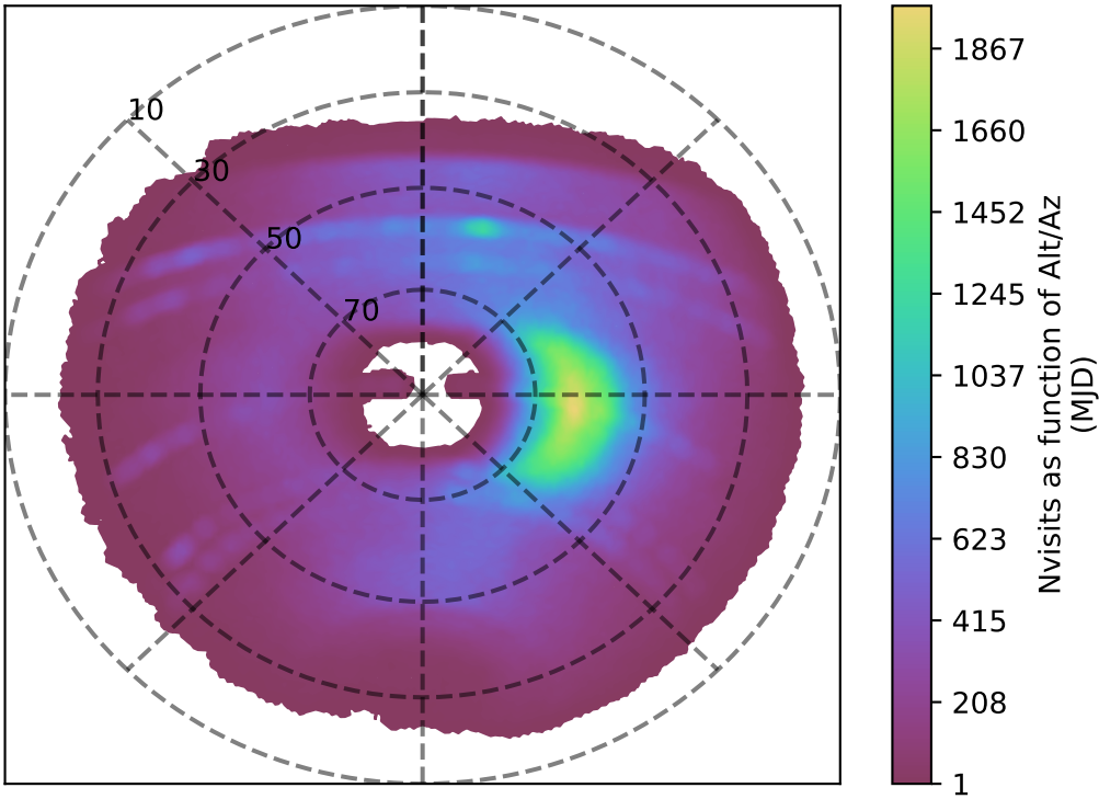
internal_u_expt60_nscale1.5v3.4_10yrs y band: Nvisits as function of Alt/Az
