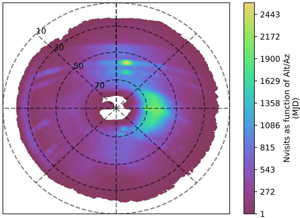
internal_u_expt60_nscale1.5v3.4_10yrs r band: Nvisits as function of Alt/Az
