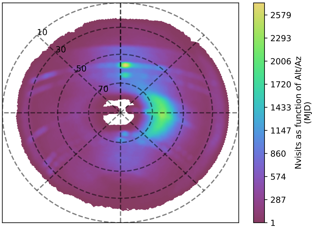
internal_u_expt60_nscale1.5v3.4_10yrs i band: Nvisits as function of Alt/Az
