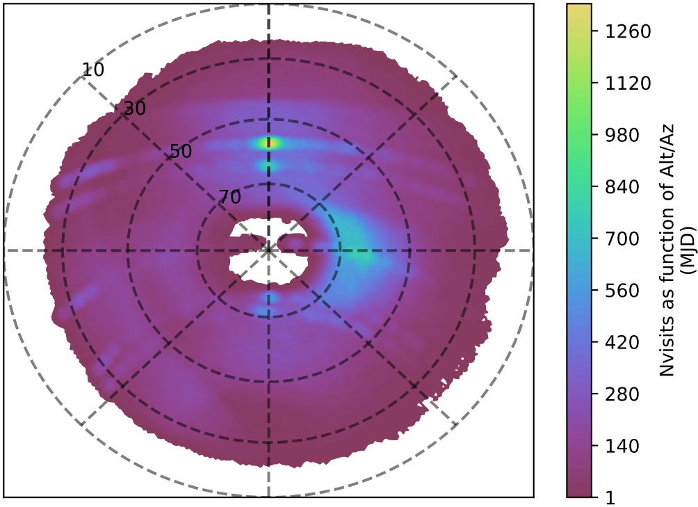
internal_u_expt60_nscale1.5v3.4_10yrs g band: Nvisits as function of Alt/Az
