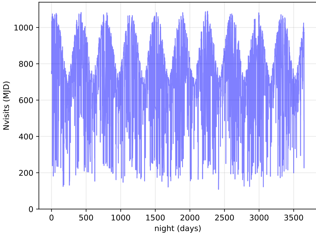
internal_u_expt60_nscale1.5v3.4_10yrs All visits: Nvisits
