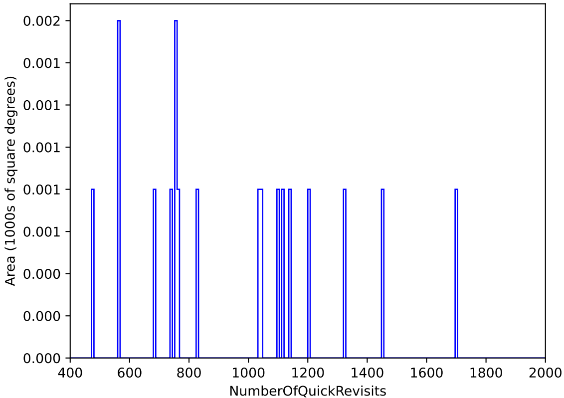
internal_u_expt60_nscale1.5v3.4_10yrs WFD: NumberOfQuickRevisits
