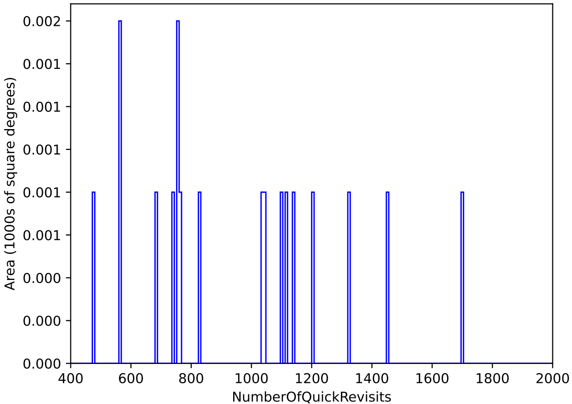
internal_u_expt60_nscale1.5v3.4_10yrs All sky: NumberOfQuickRevisits
