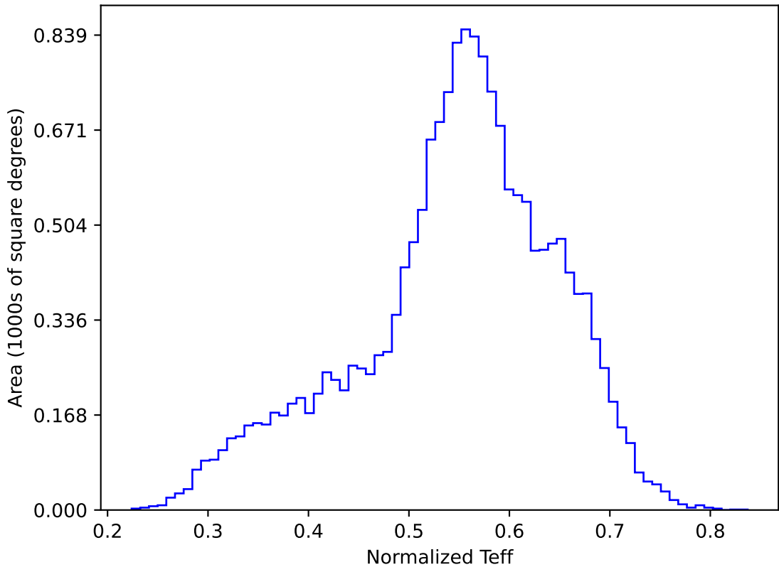
internal_u_expt60_nscale1.5v3.4_10yrs WFD y band: Normalized Teff
