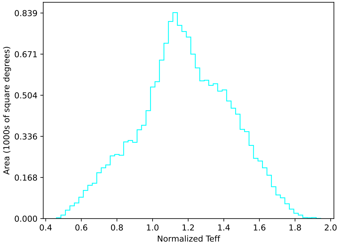
internal_u_expt60_nscale1.5v3.4_10yrs WFD u band: Normalized Teff
