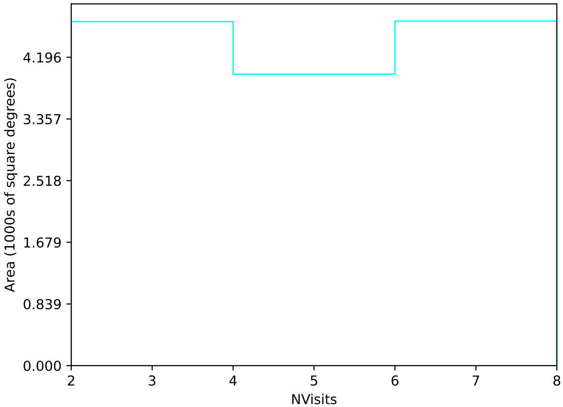
internal_u_expt60_nscale1.5v3.4_10yrs Yr 3-4 u band: NVisits
