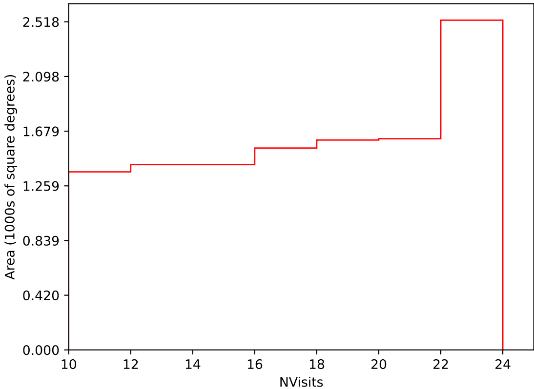
internal_u_expt60_nscale1.5v3.4_10yrs Yr 3-4 i band: NVisits
