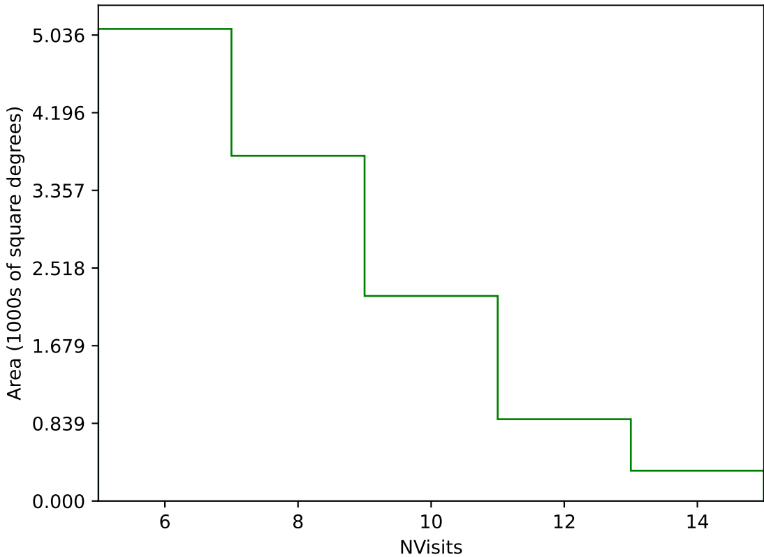
internal_u_expt60_nscale1.5v3.4_10yrs Yr 3-4 g band: NVisits
