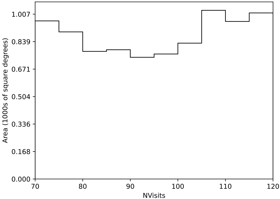
internal_u_expt60_nscale1.5v3.4_10yrs Yr 3-4 all bands: NVisits
