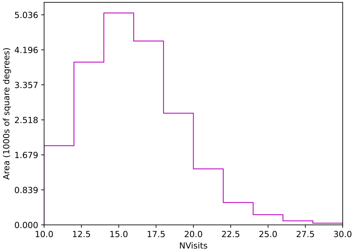
internal_u_expt60_nscale1.5v3.4_10yrs Yr 1 z band: NVisits
