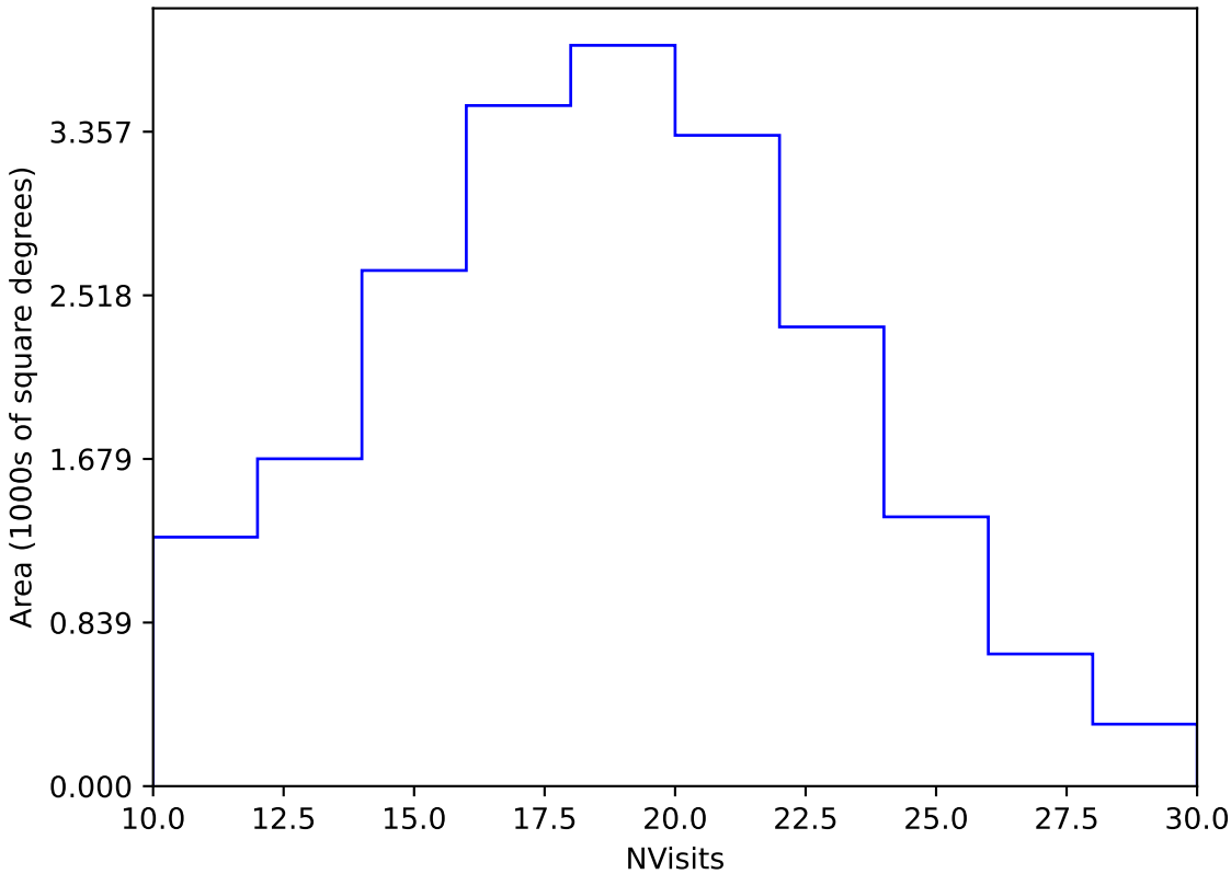
internal_u_expt60_nscale1.5v3.4_10yrs Yr 1 y band: NVisits
