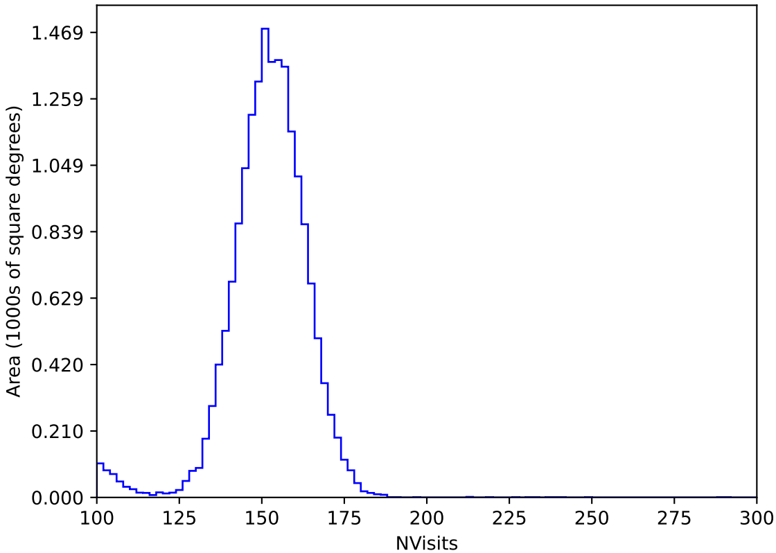
internal_u_expt60_nscale1.5v3.4_10yrs WFD y band: NVisits
