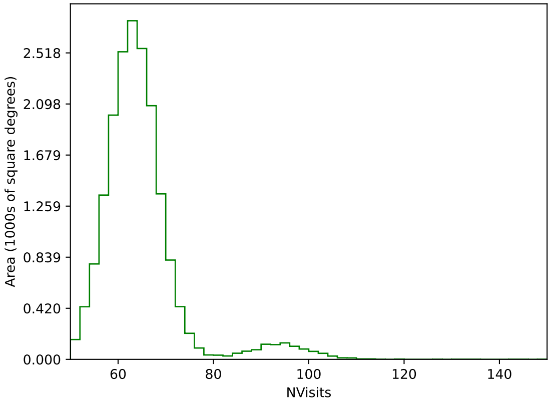
internal_u_expt60_nscale1.5v3.4_10yrs WFD g band: NVisits
