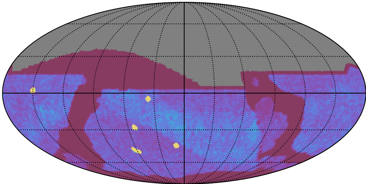
internal_u_expt60_nscale1.5v3.4_10yrs All sky z band: NVisits
