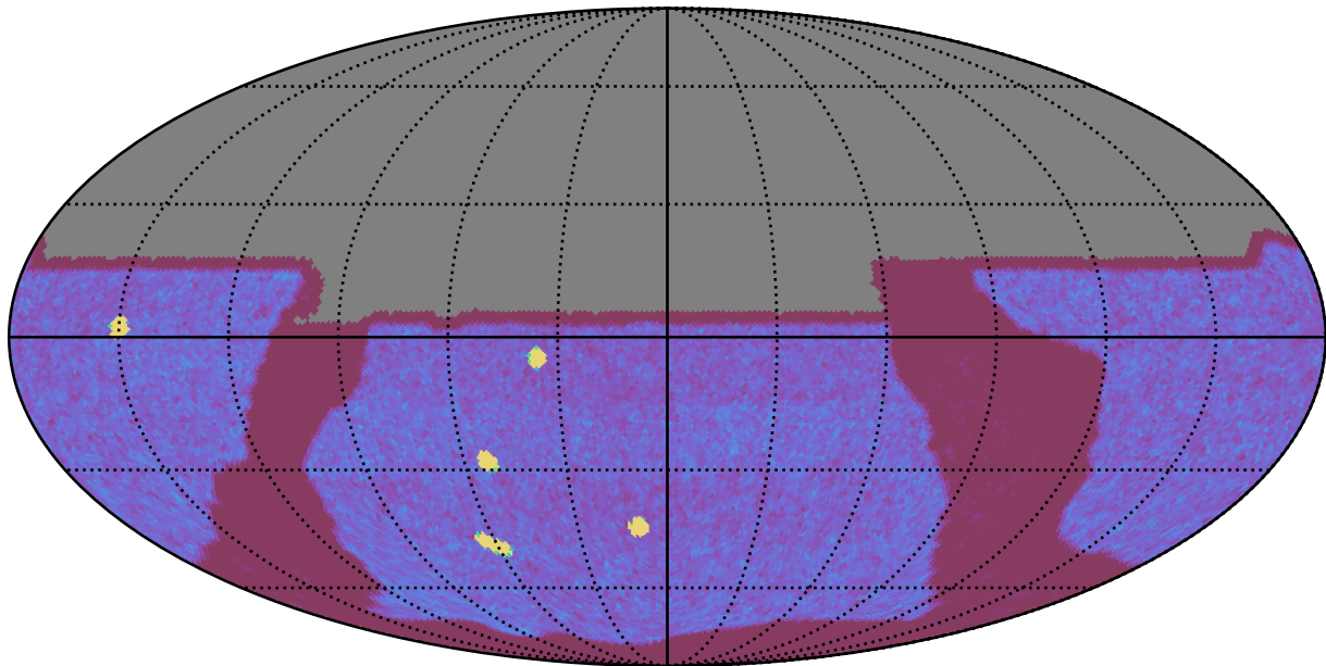
internal_u_expt60_nscale1.5v3.4_10yrs All sky y band: NVisits
