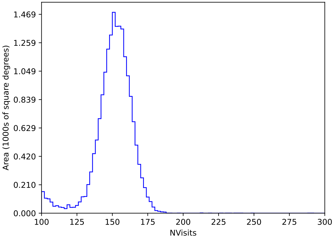
internal_u_expt60_nscale1.5v3.4_10yrs All sky y band: NVisits
