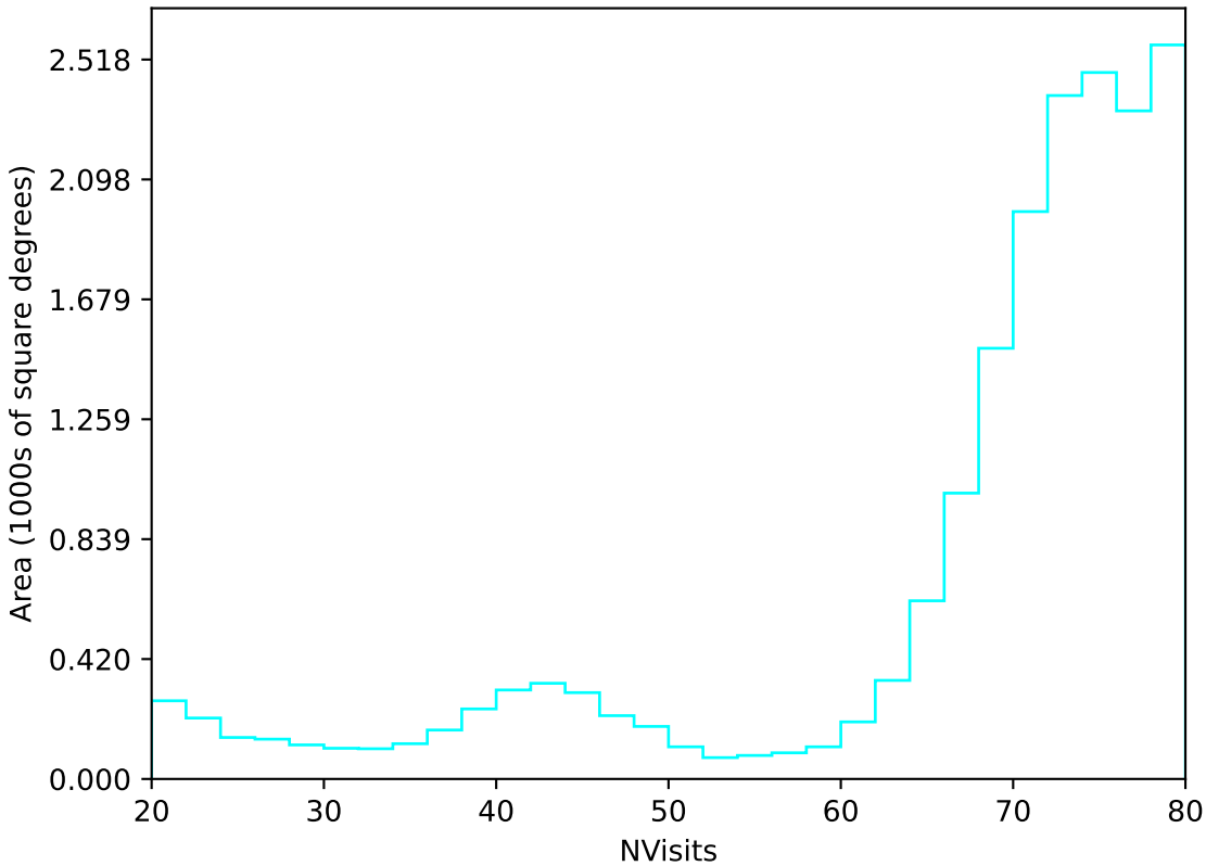
internal_u_expt60_nscale1.5v3.4_10yrs All sky u band: NVisits
