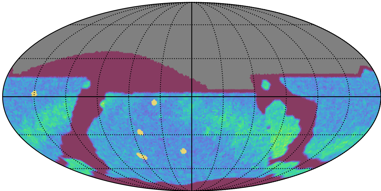
internal_u_expt60_nscale1.5v3.4_10yrs All sky r band: NVisits
