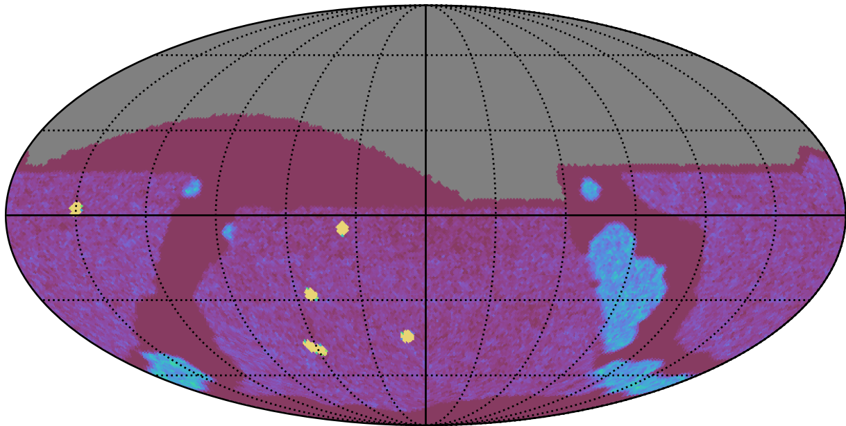
internal_u_expt60_nscale1.5v3.4_10yrs All sky g band: NVisits
