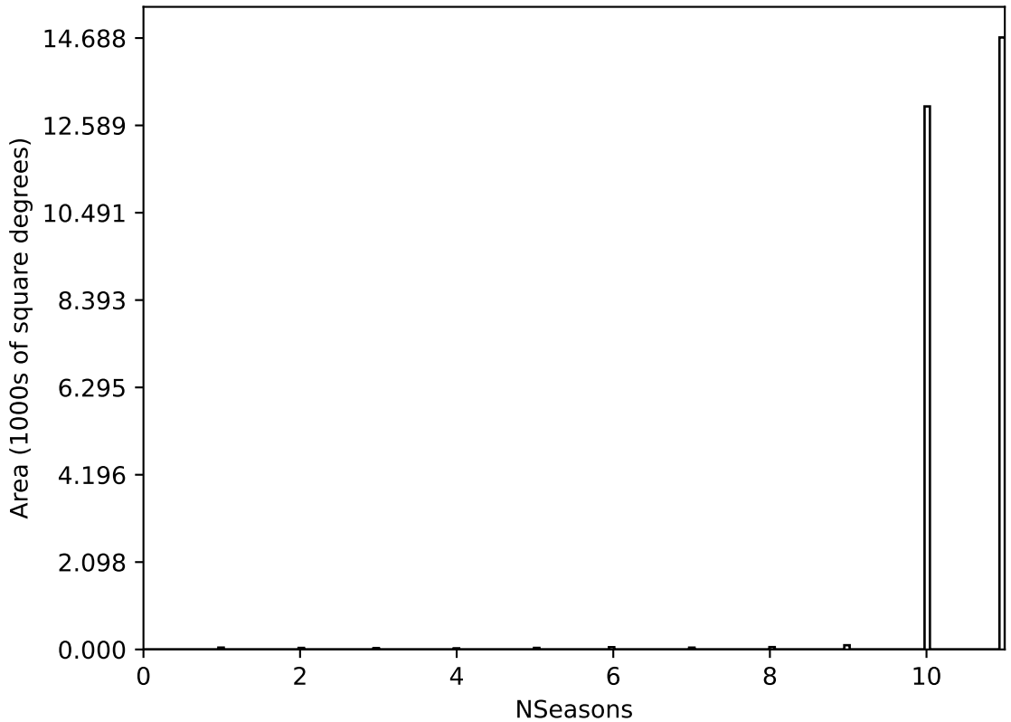
internal_u_expt60_nscale1.5v3.4_10yrs All sky all bands: NSeasons
