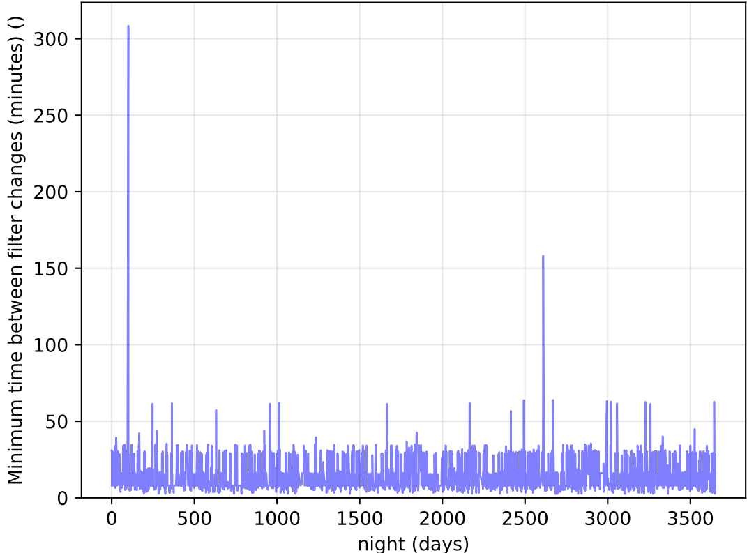
internal_u_expt60_nscale1.5v3.4_10yrs Per Night: Minimum time between filter changes (minutes)
