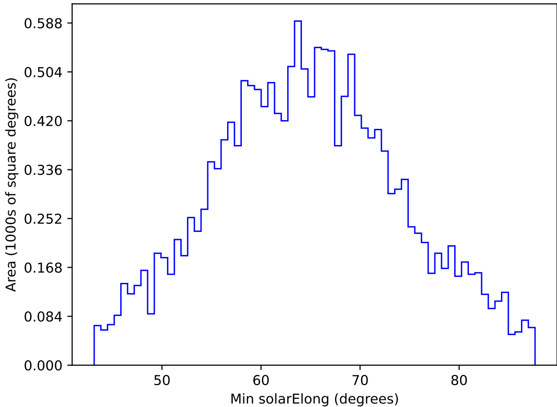
internal_u_expt60_nscale1.5v3.4_10yrs WFD y band: Min solarElong
