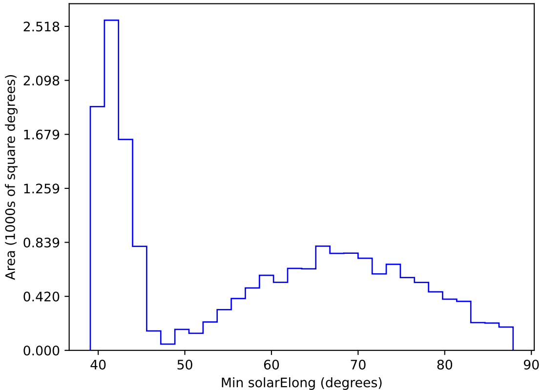
internal_u_expt60_nscale1.5v3.4_10yrs WFD r band: Min solarElong
