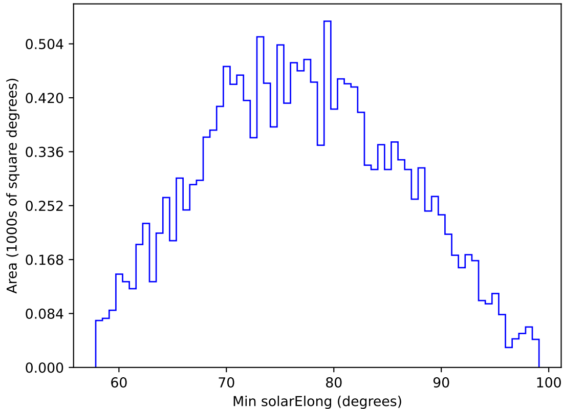
internal_u_expt60_nscale1.5v3.4_10yrs WFD g band: Min solarElong
