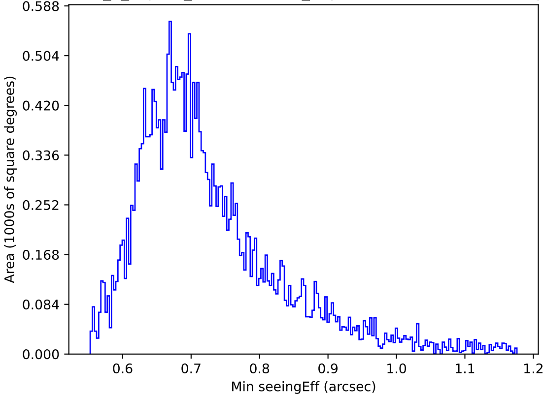
internal_u_expt60_nscale1.5v3.4_10yrs Yr 1 z band: Min seeingEff
