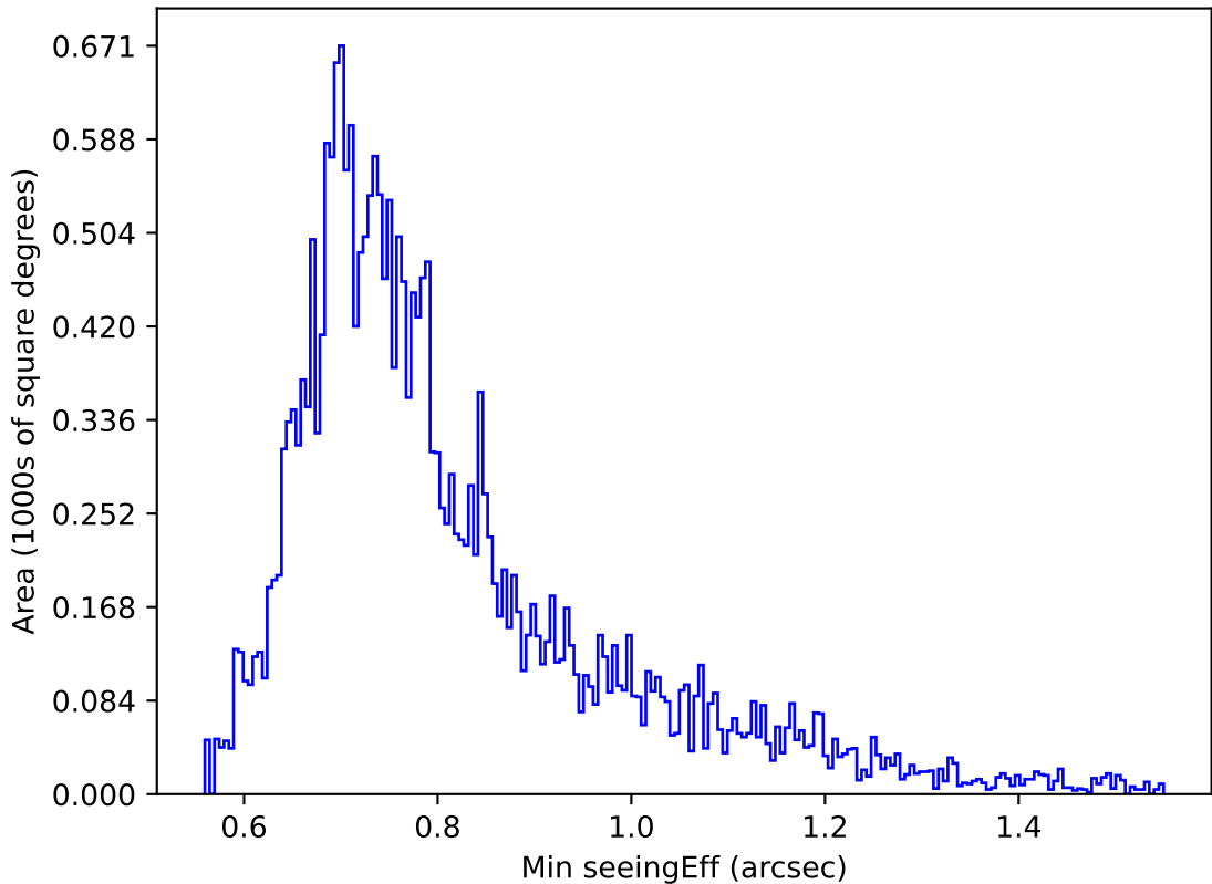
internal_u_expt60_nscale1.5v3.4_10yrs Yr 1 g band: Min seeingEff
