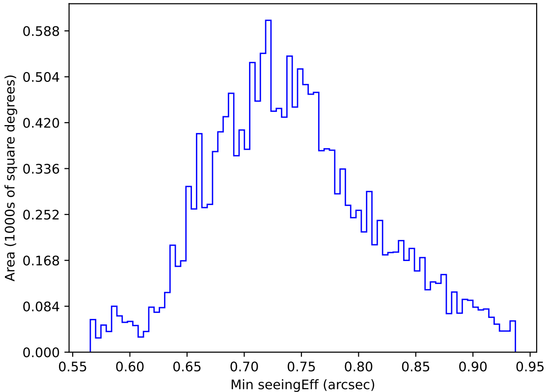
internal_u_expt60_nscale1.5v3.4_10yrs WFD u band: Min seeingEff
