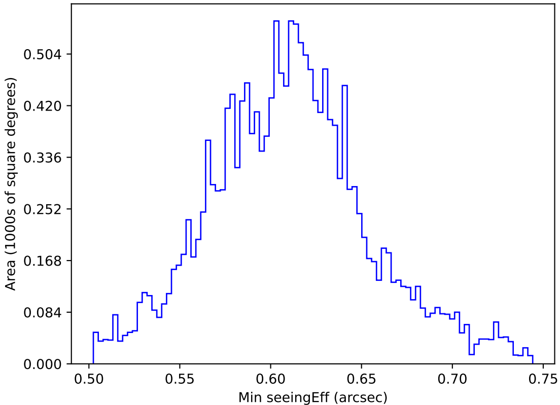
internal_u_expt60_nscale1.5v3.4_10yrs WFD r band: Min seeingEff
