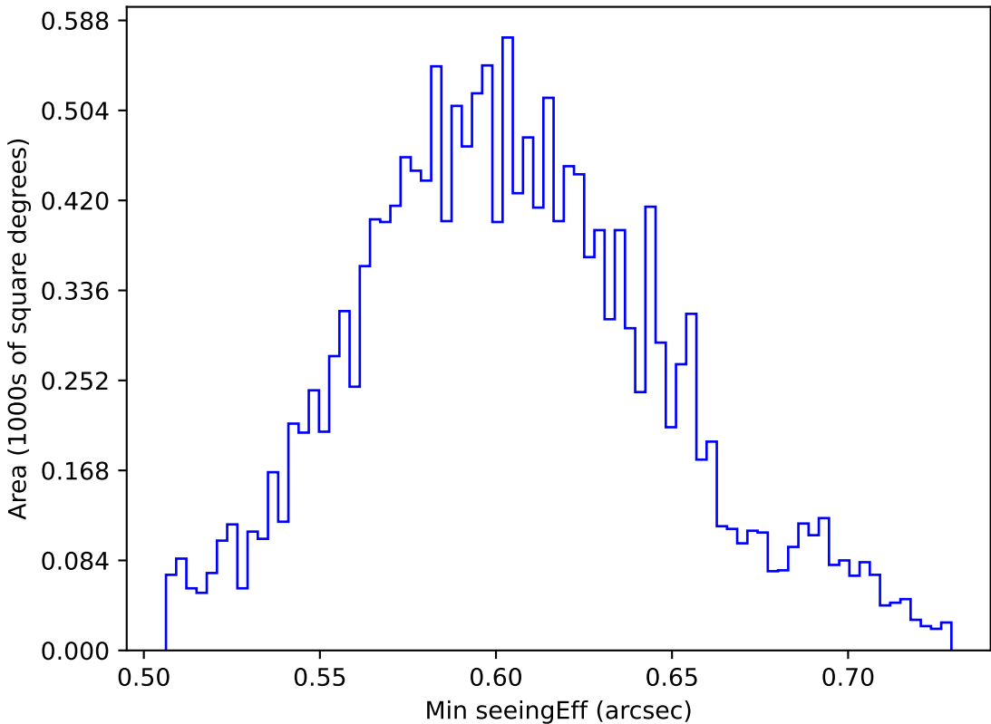
internal_u_expt60_nscale1.5v3.4_10yrs WFD i band: Min seeingEff
