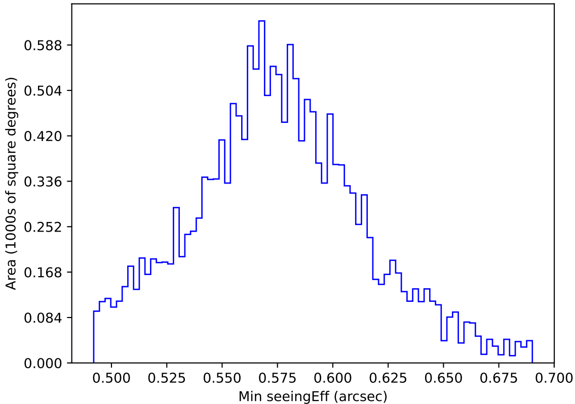
internal_u_expt60_nscale1.5v3.4_10yrs WFD all bands: Min seeingEff
