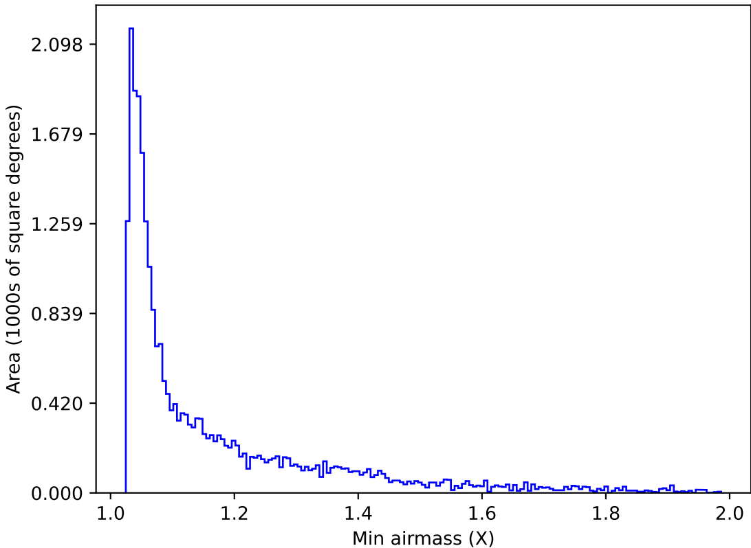
internal_u_expt60_nscale1.5v3.4_10yrs Yr 1 z band: Min airmass
