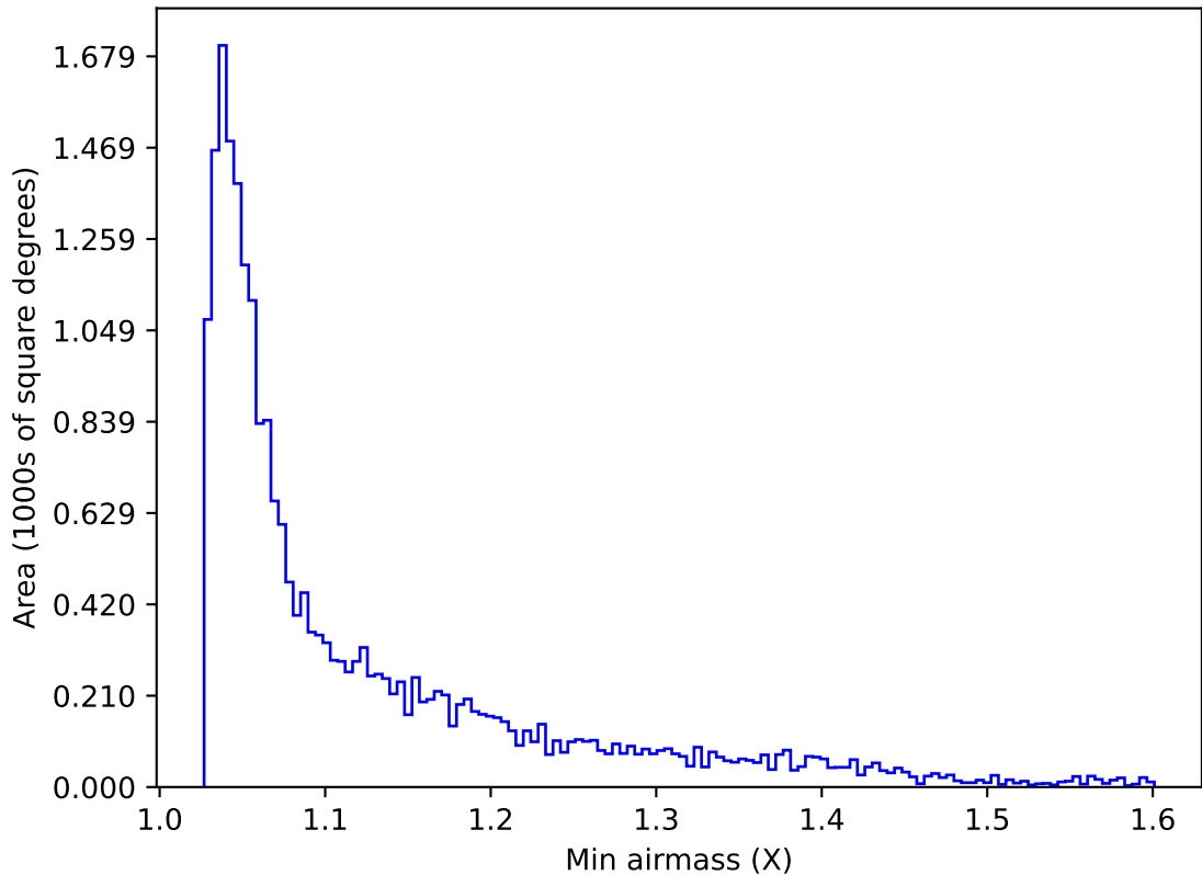
internal_u_expt60_nscale1.5v3.4_10yrs Yr 1 y band: Min airmass
