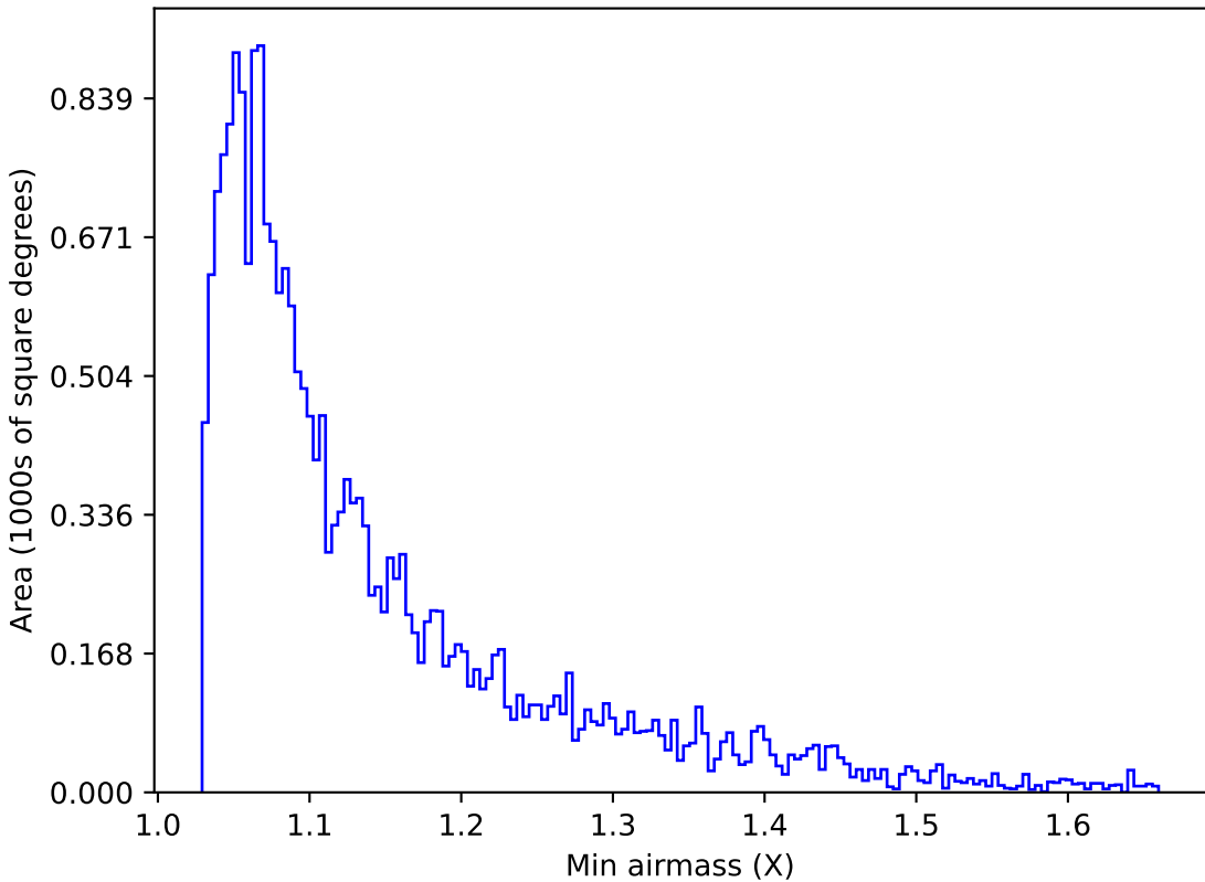
internal_u_expt60_nscale1.5v3.4_10yrs Yr 1 u band: Min airmass
