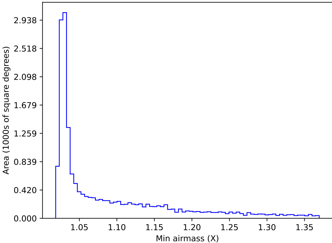
internal_u_expt60_nscale1.5v3.4_10yrs WFD z band: Min airmass
