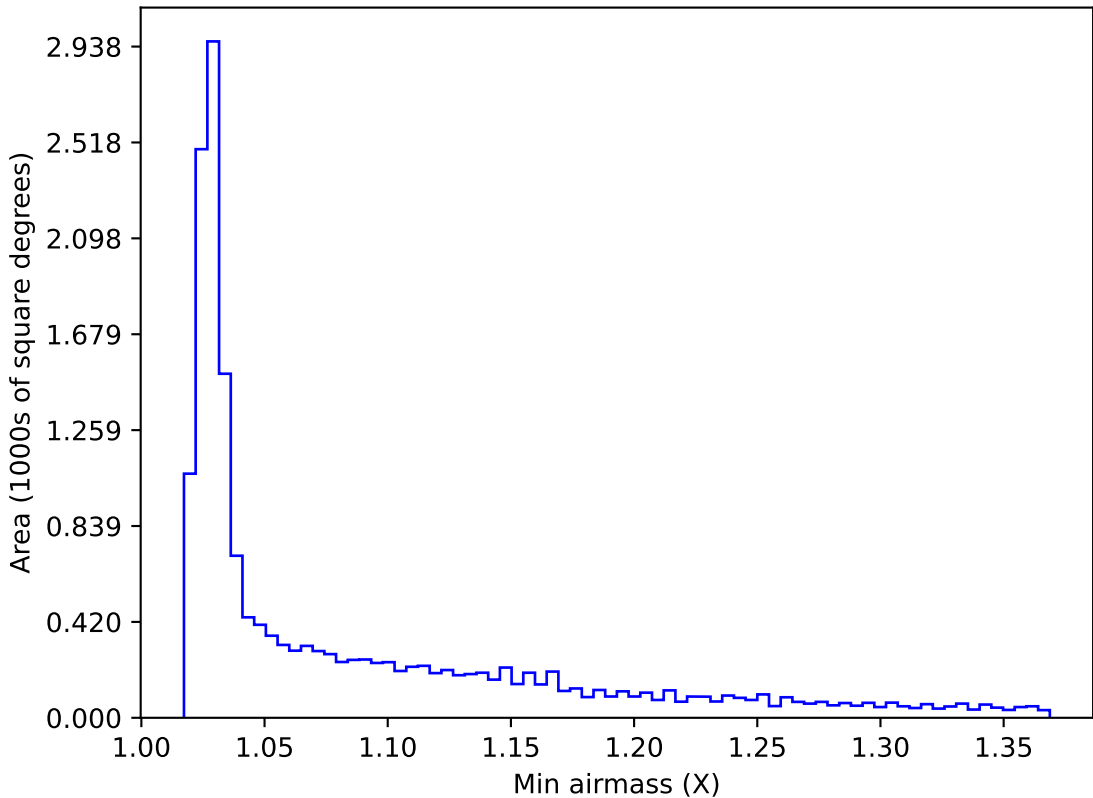
internal_u_expt60_nscale1.5v3.4_10yrs WFD r band: Min airmass
