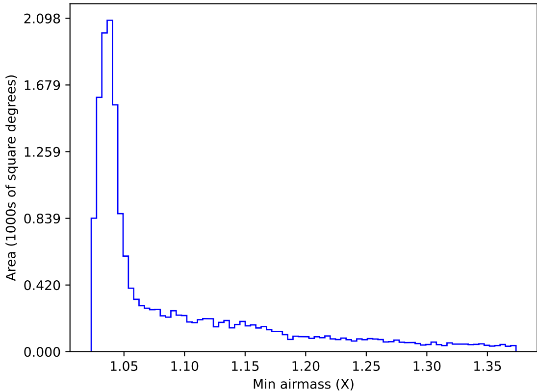
internal_u_expt60_nscale1.5v3.4_10yrs WFD g band: Min airmass
