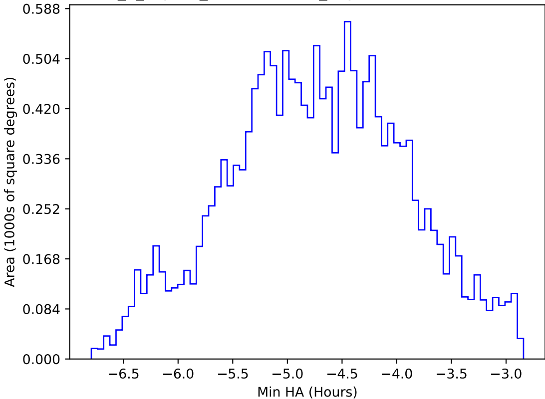
internal_u_expt60_nscale1.5v3.4_10yrs WFD all bands: Min HA
