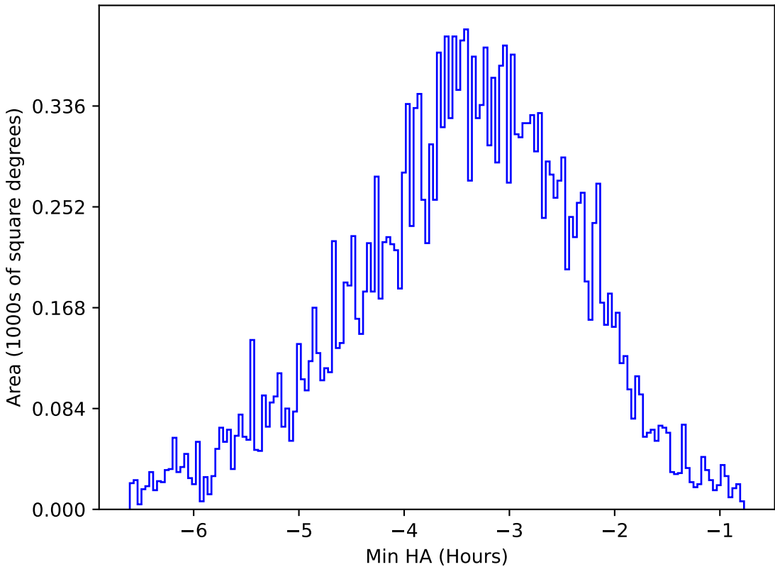
internal_u_expt60_nscale1.5v3.4_10yrs All sky y band: Min HA
