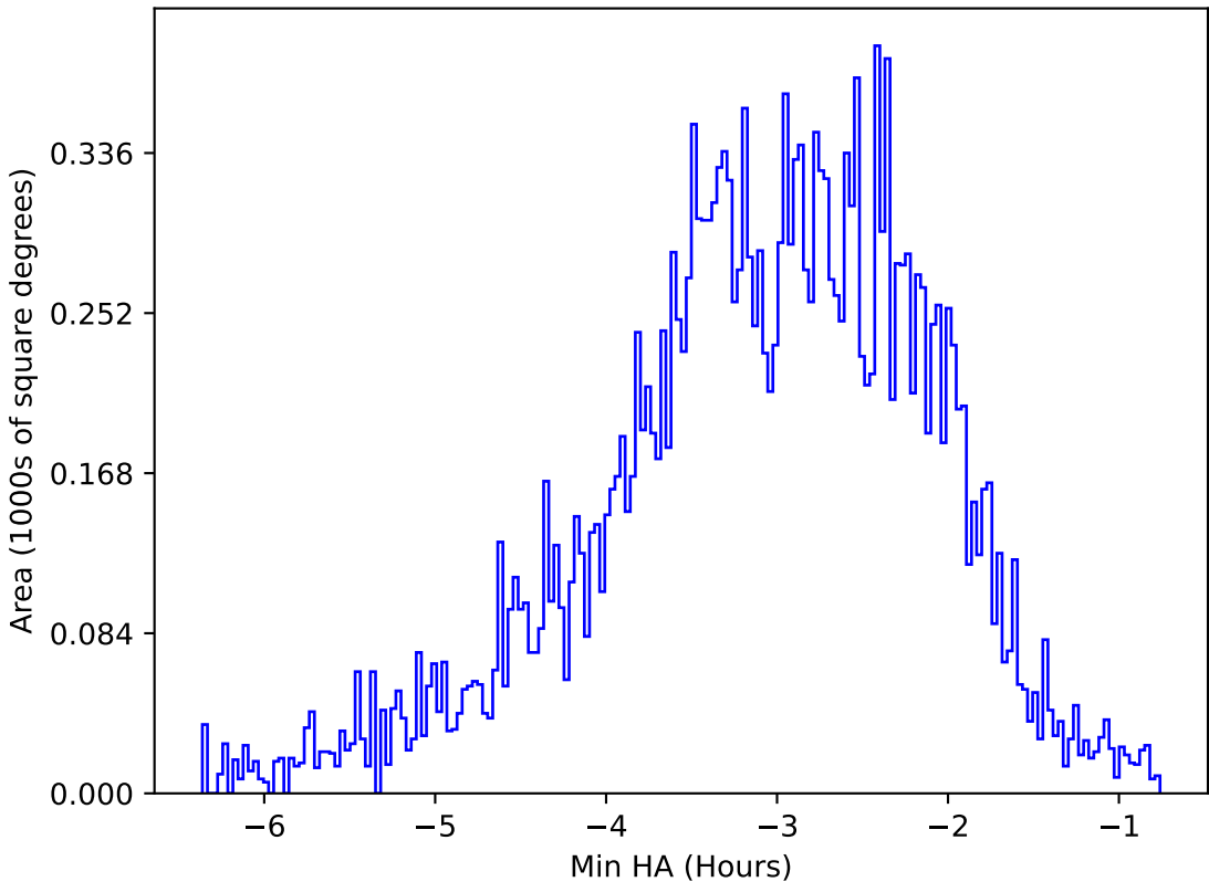
internal_u_expt60_nscale1.5v3.4_10yrs All sky u band: Min HA
