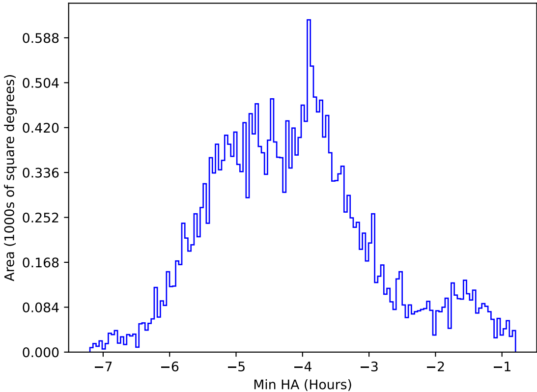
internal_u_expt60_nscale1.5v3.4_10yrs All sky r band: Min HA
