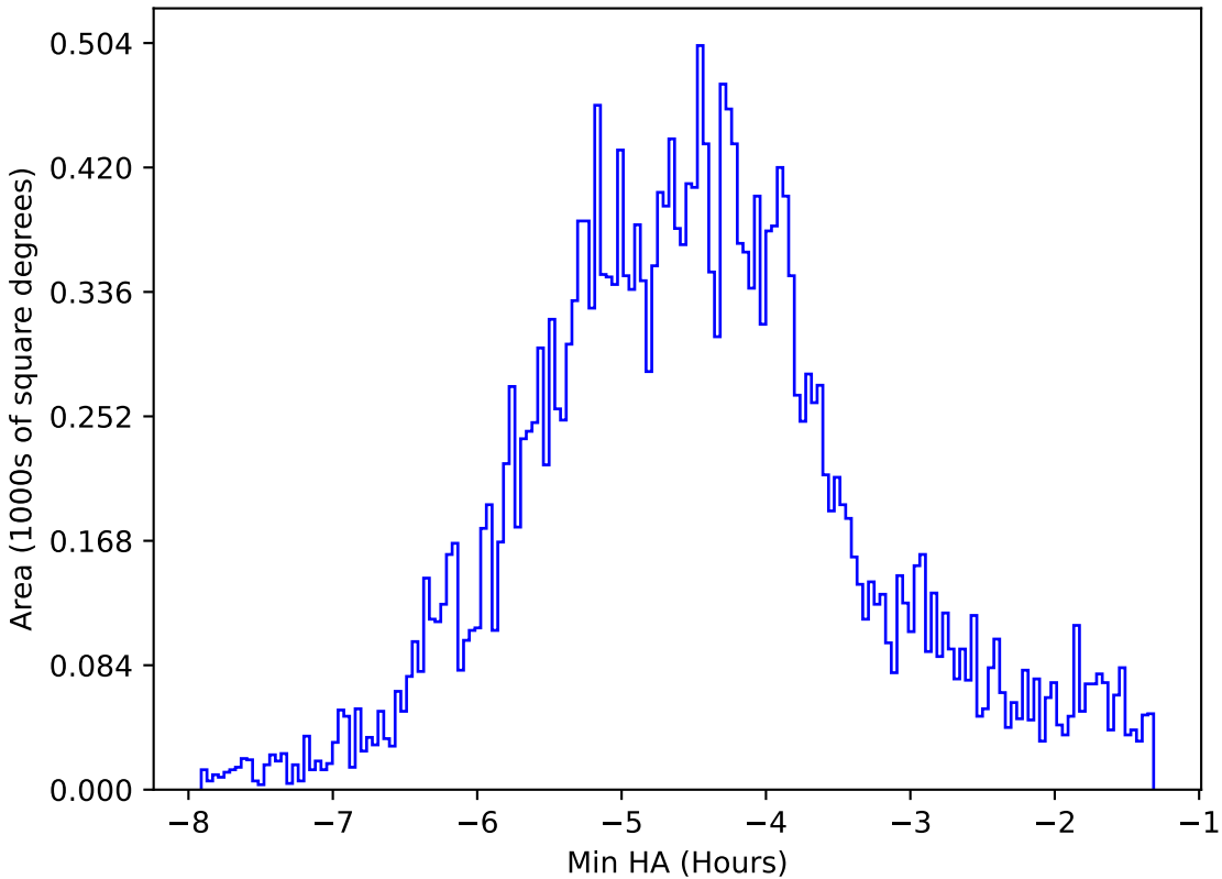
internal_u_expt60_nscale1.5v3.4_10yrs All sky all bands: Min HA
