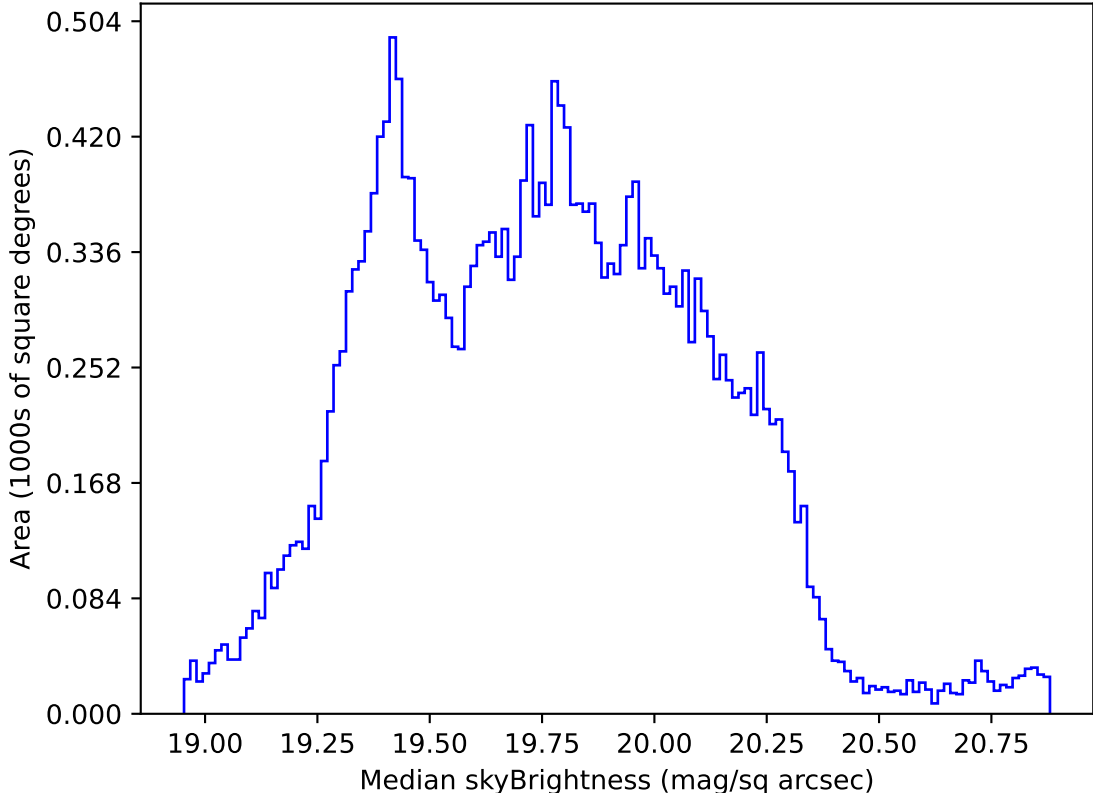
internal_u_expt60_nscale1.5v3.4_10yrs Yr 1 all bands: Median skyBrightness
