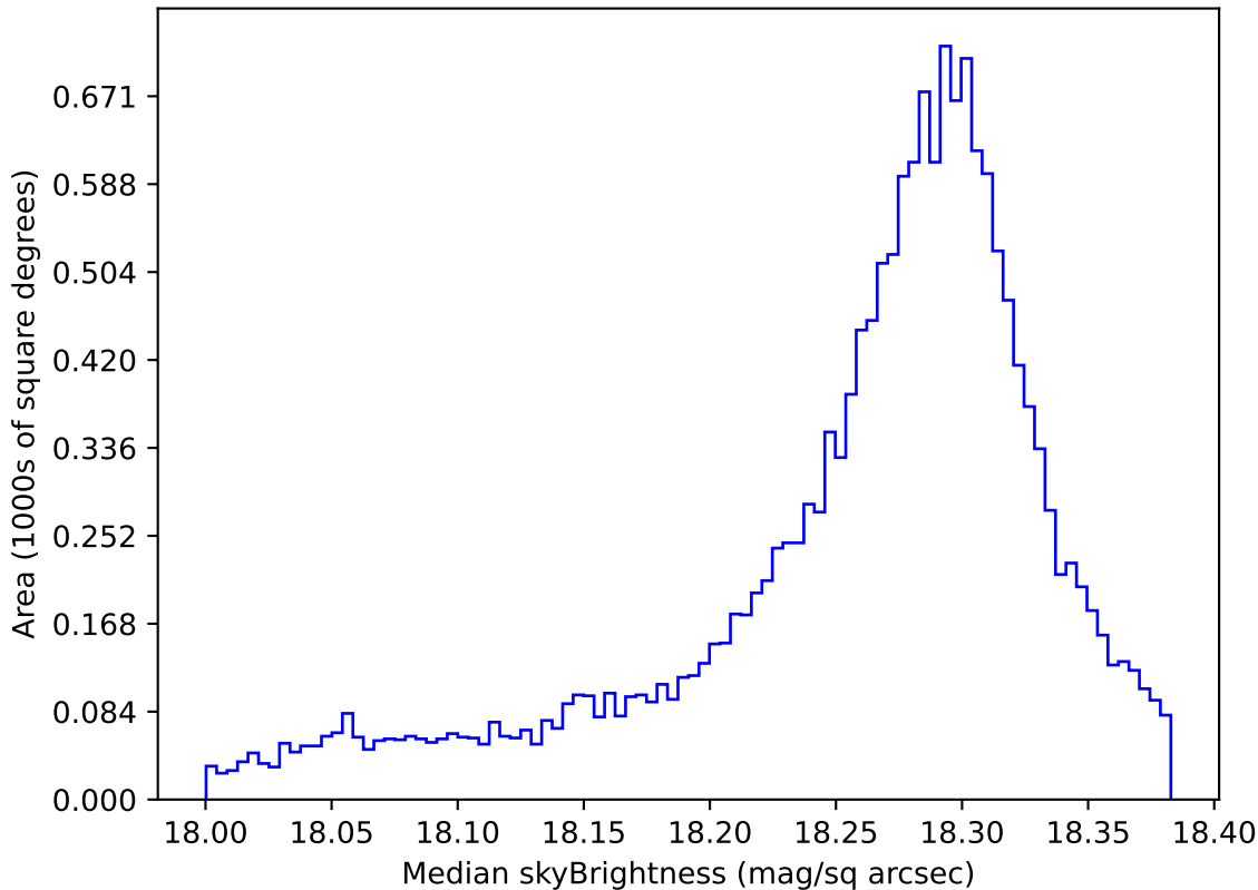
internal_u_expt60_nscale1.5v3.4_10yrs WFD y band: Median skyBrightness
