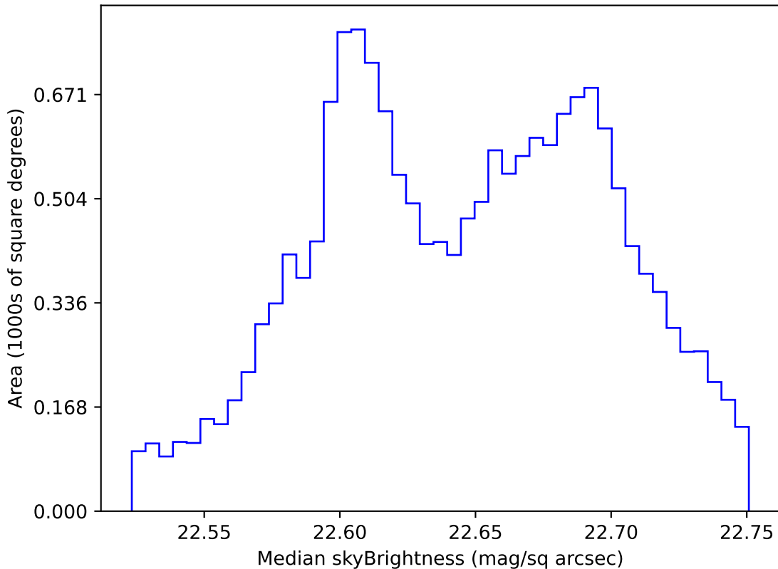
internal_u_expt60_nscale1.5v3.4_10yrs WFD u band: Median skyBrightness
