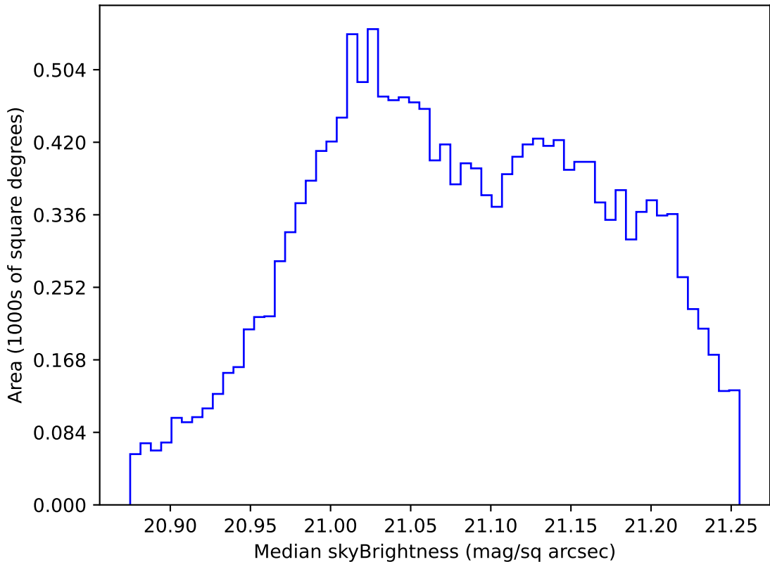
internal_u_expt60_nscale1.5v3.4_10yrs WFD r band: Median skyBrightness
